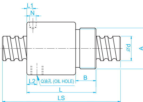
d \geq 16 (Internal circulation type) 內循環
