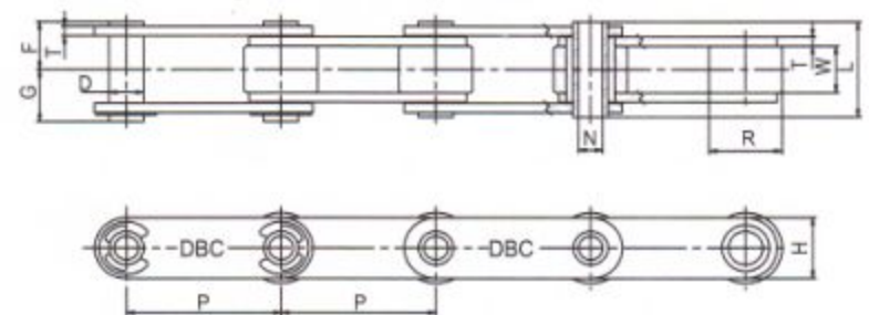
Roller Type
