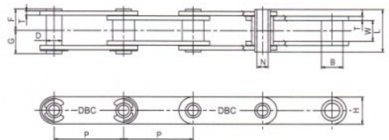
Bushed Type
