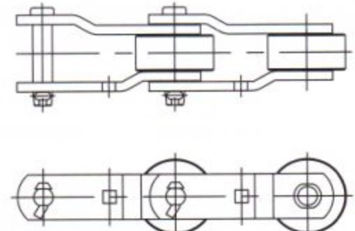
Bottle-Washer Chain [ 瓶型清洗链条 ]
