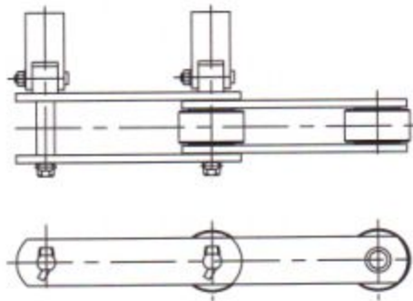
Hinged Chain [ 铰接链 ]
