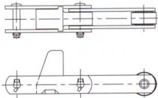
Dog Chain [ 挡板链条 ]
