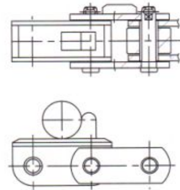
Dog Chain [ 挡板链条 ]
