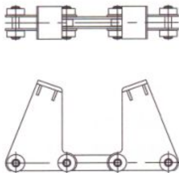
Saddle Chain [ 鞍板链条 ]
