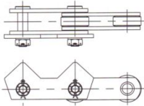
Chain for section steel transportation Chain [ 钢材运输链 ]
