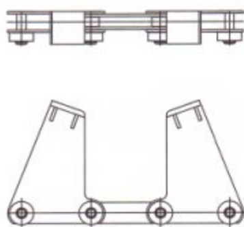
Saddle Chain [ 鞍板链条 ]
