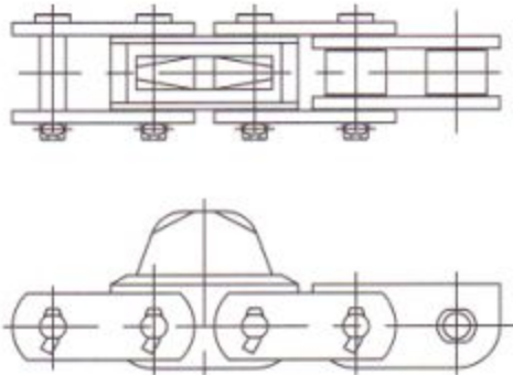
Flight Chain [ 梯级链条 ]
