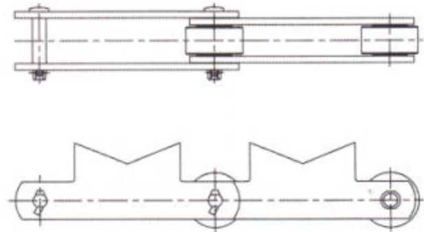
Scraper Chain [ 刮板链条 ]
